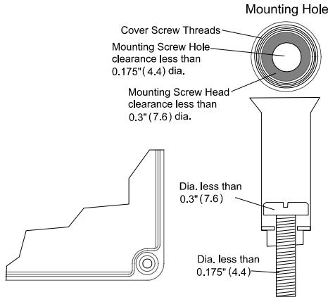
Figure 31. Wall Mounting Screw
